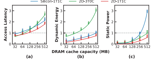
Fig. 9: (a) Access latency, (b) dynamic energy, and (c) static power of DRAM caches based on different cell structures and materials as capacity increases. Values are normalized to the 32MB SRAM cache. The scatter points represent feasible configurations identified during the design space exploration.
