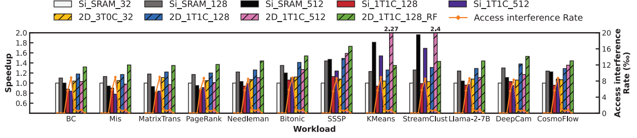
Fig. 10: Performance and access interference rate comparison of several DRAM cache configurations for common GPU workloads. The shaded regions denote configurations based on 2D-material DRAM caches.
